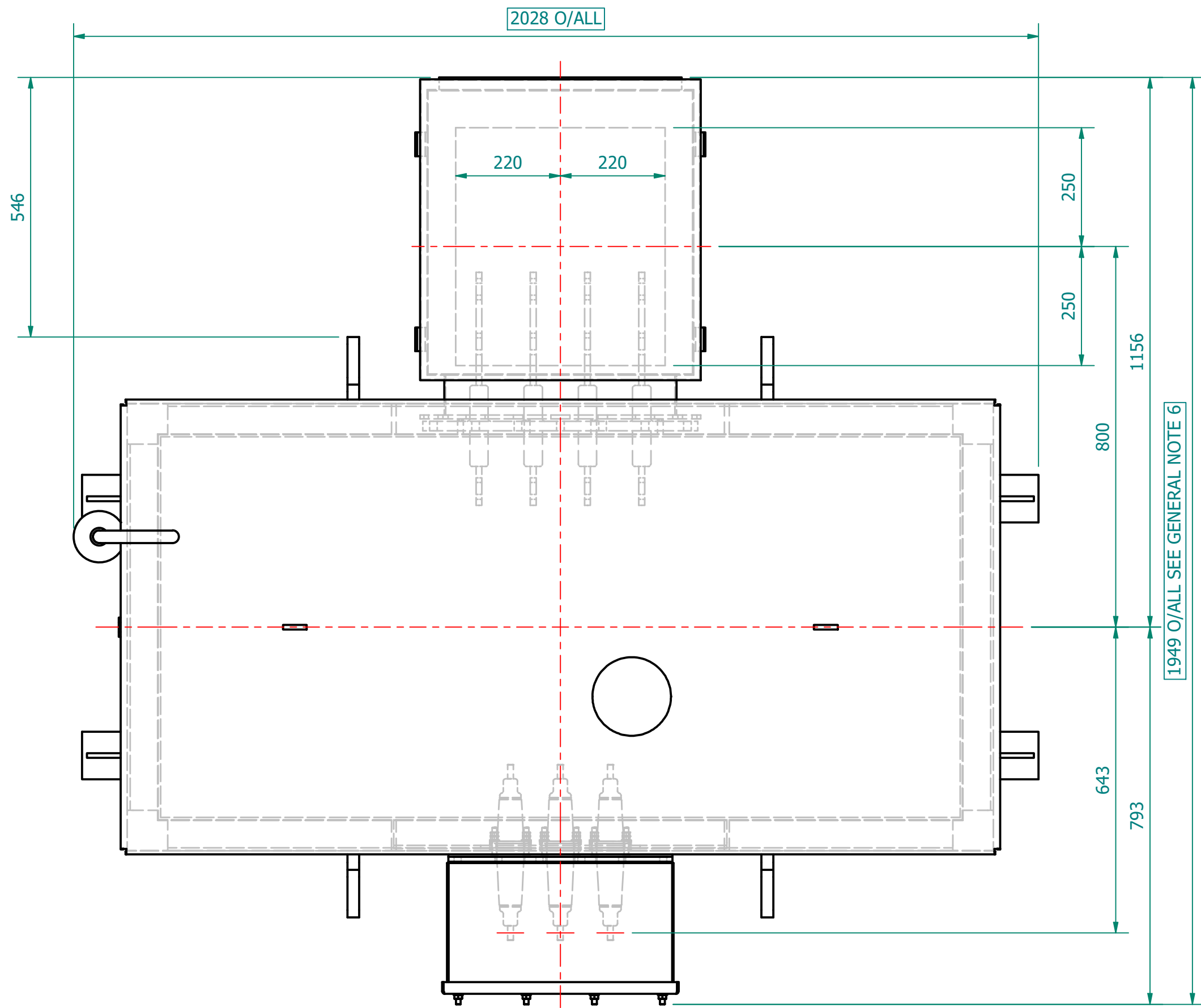
PLAN VIEW
