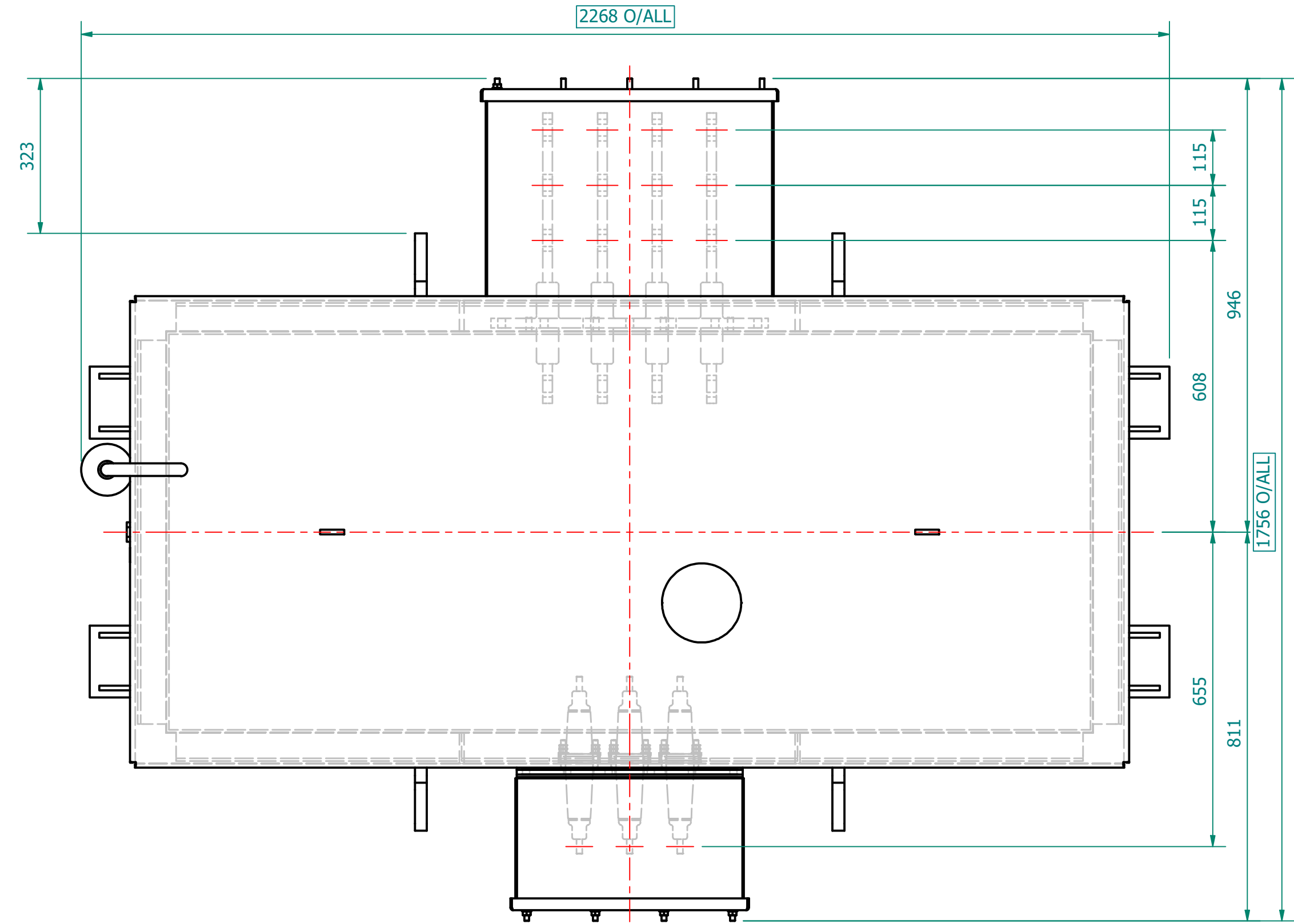
PLAN VIEW
