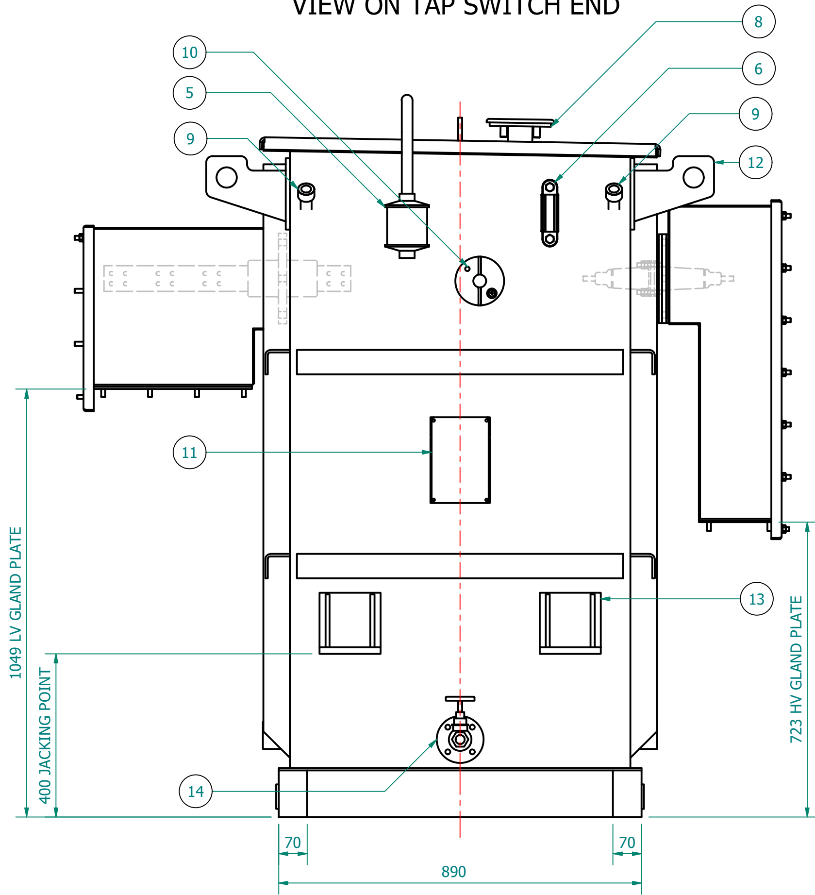
VIEW ON TAP SWITCH END
