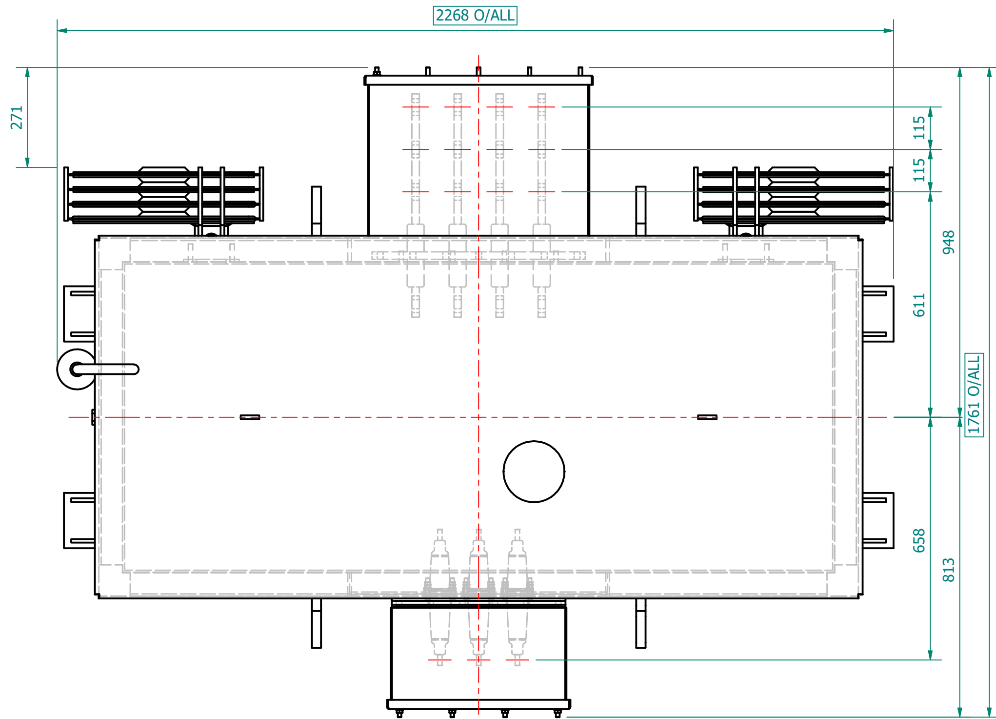
PLAN VIEW
