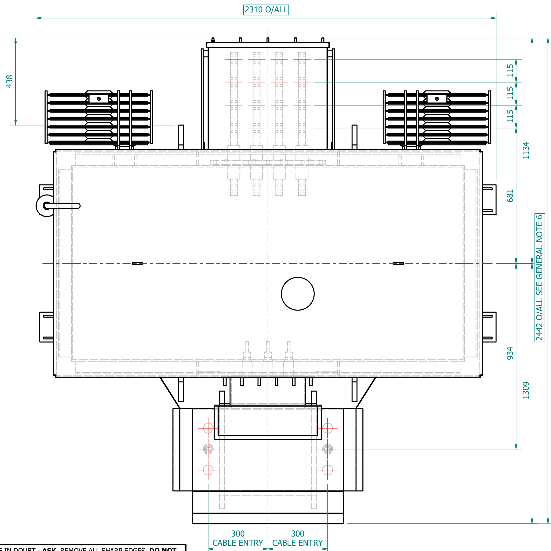
PLAN VIEW
