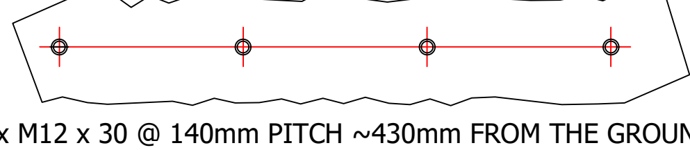
VIEW OF LV SIDE - CABLE CLEAT STUDS CABLES MUST BE SUPPORTED IN ACCORDANCE WITH - CURRENT IET Wiring Regulations BS7671 & IEC 61914
