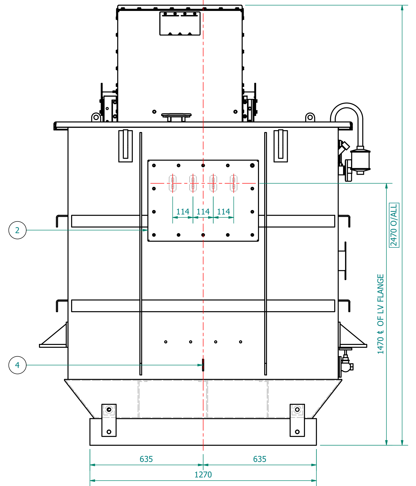
VIEW ON LV SIDE PHASE ROTATION 2W 2V 2U 2N
