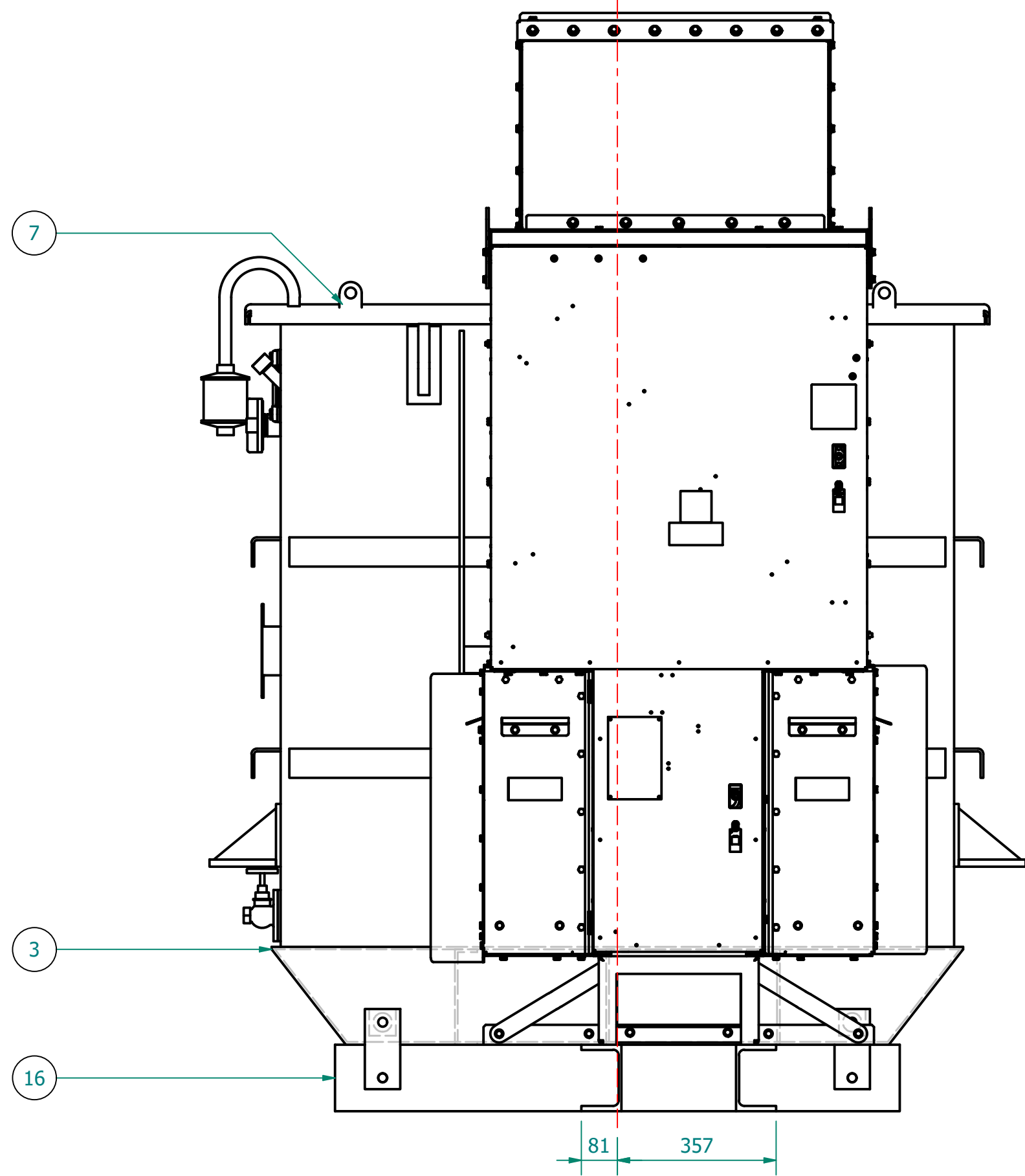
VIEW ON HV SIDE PHASE ROTATION 1U 1V 1W
