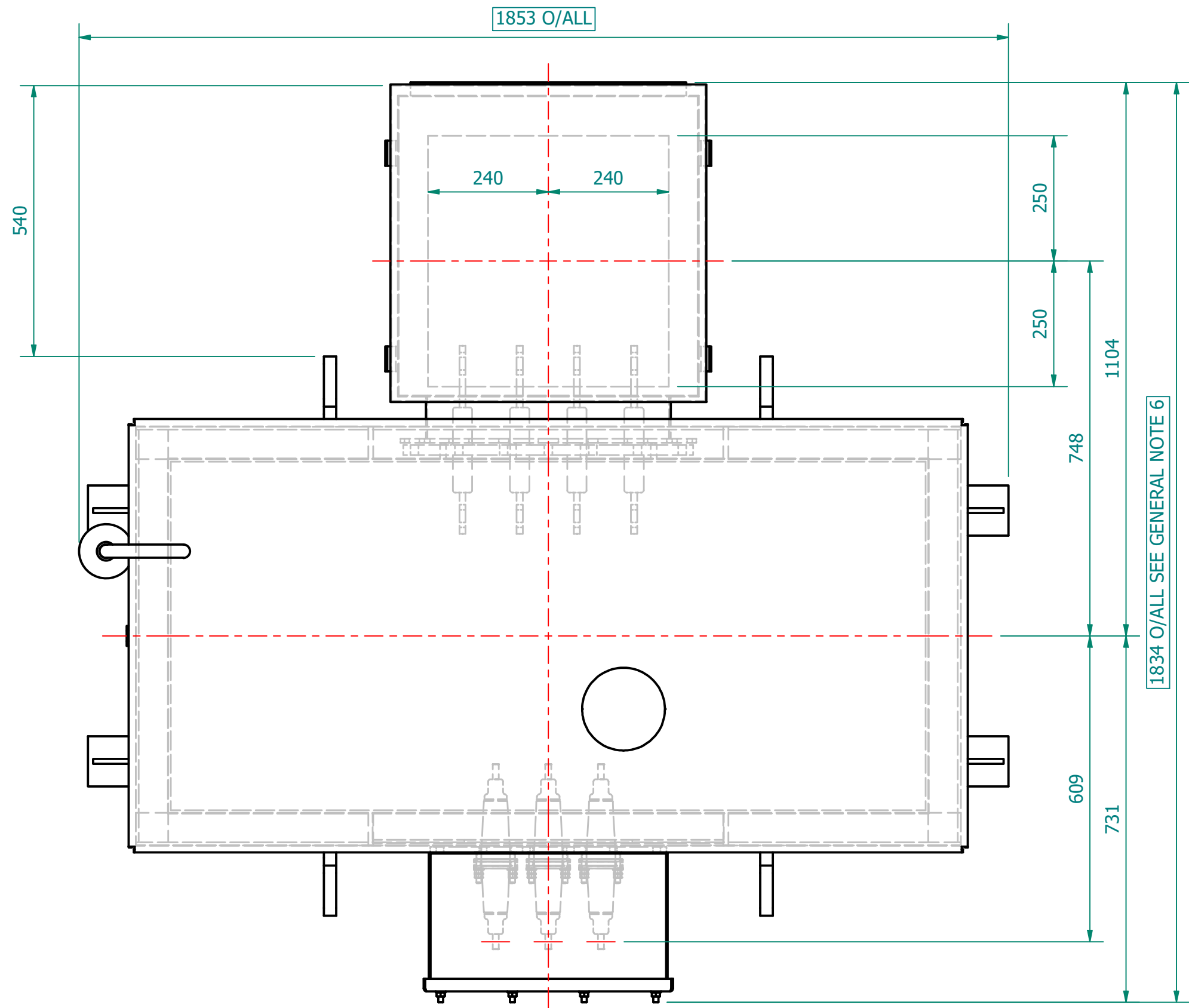
PLAN VIEW
