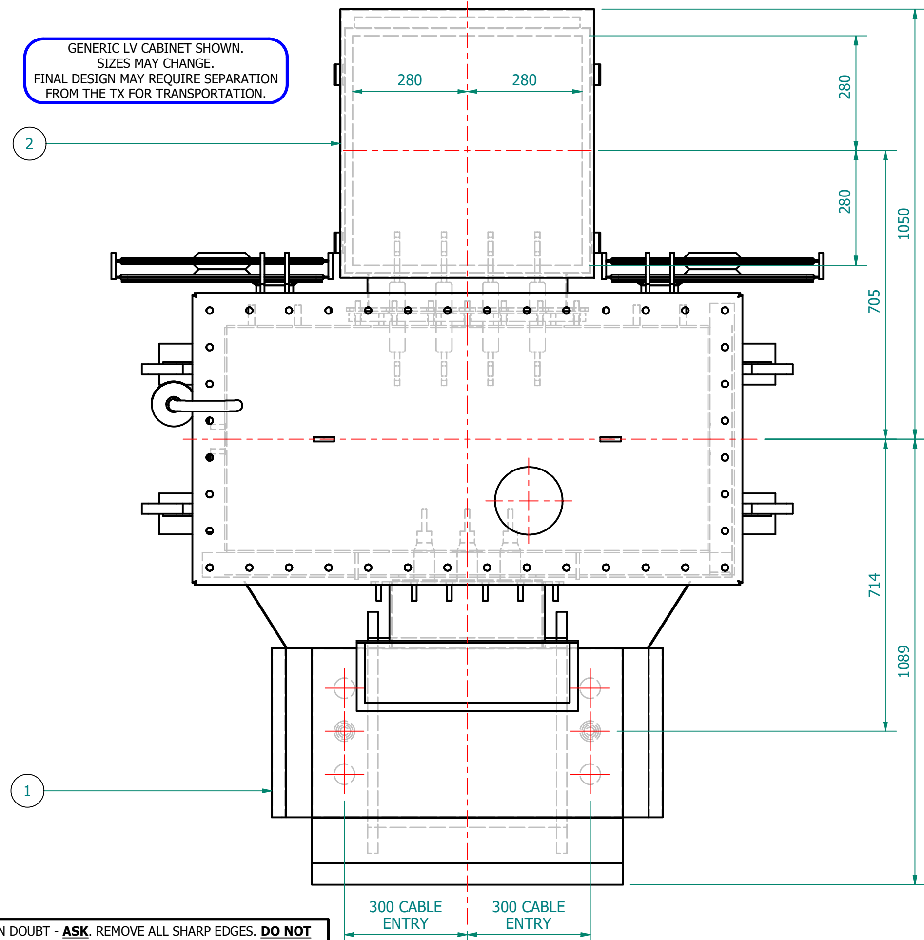
PLAN VIEW
