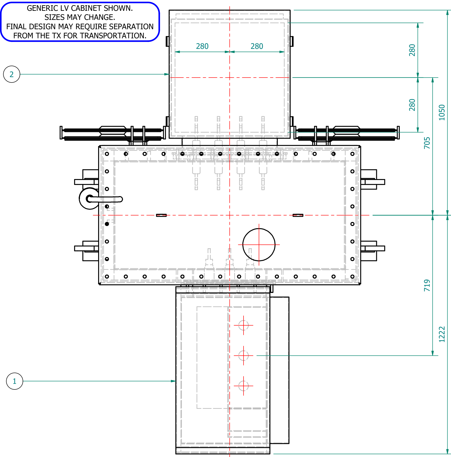
PLAN VIEW
